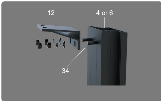
96° Column &amp; Rafter Connector Installation
