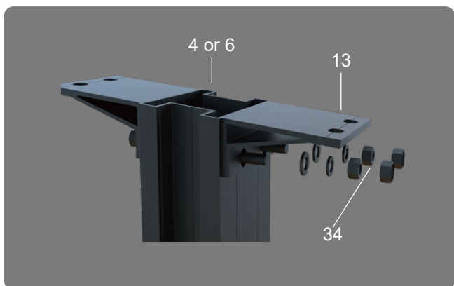
84° Column &amp; Rafter Connector Installation
