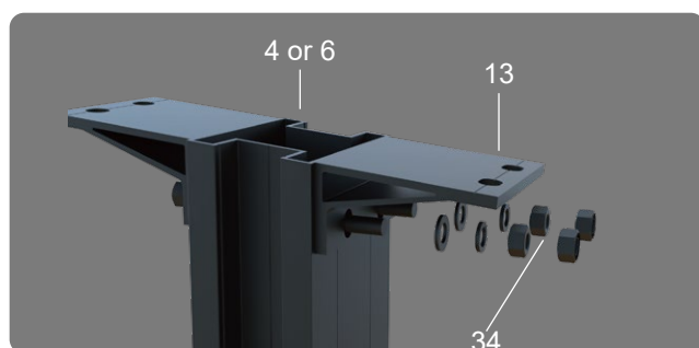
96° & 84° Column & Rafter Connector Installation
