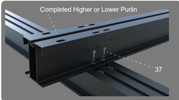
Before Installation
