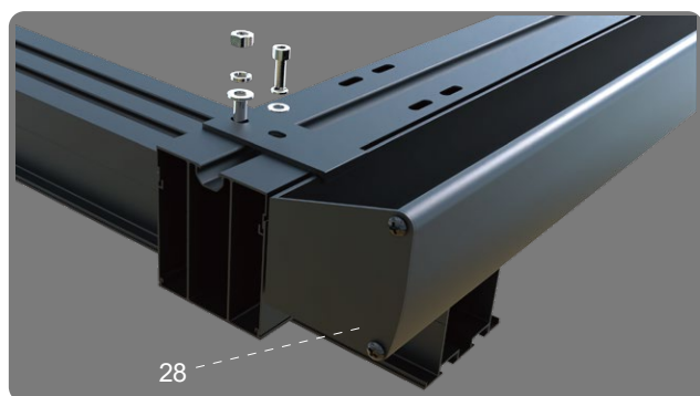
Gutter Completion
