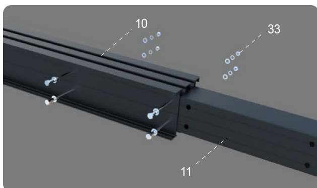
Before Installation
