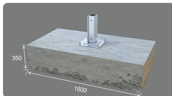
After Installation
