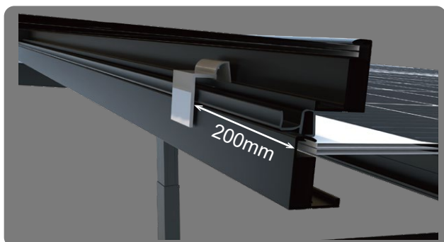
Position Diagram of weather seal tap
