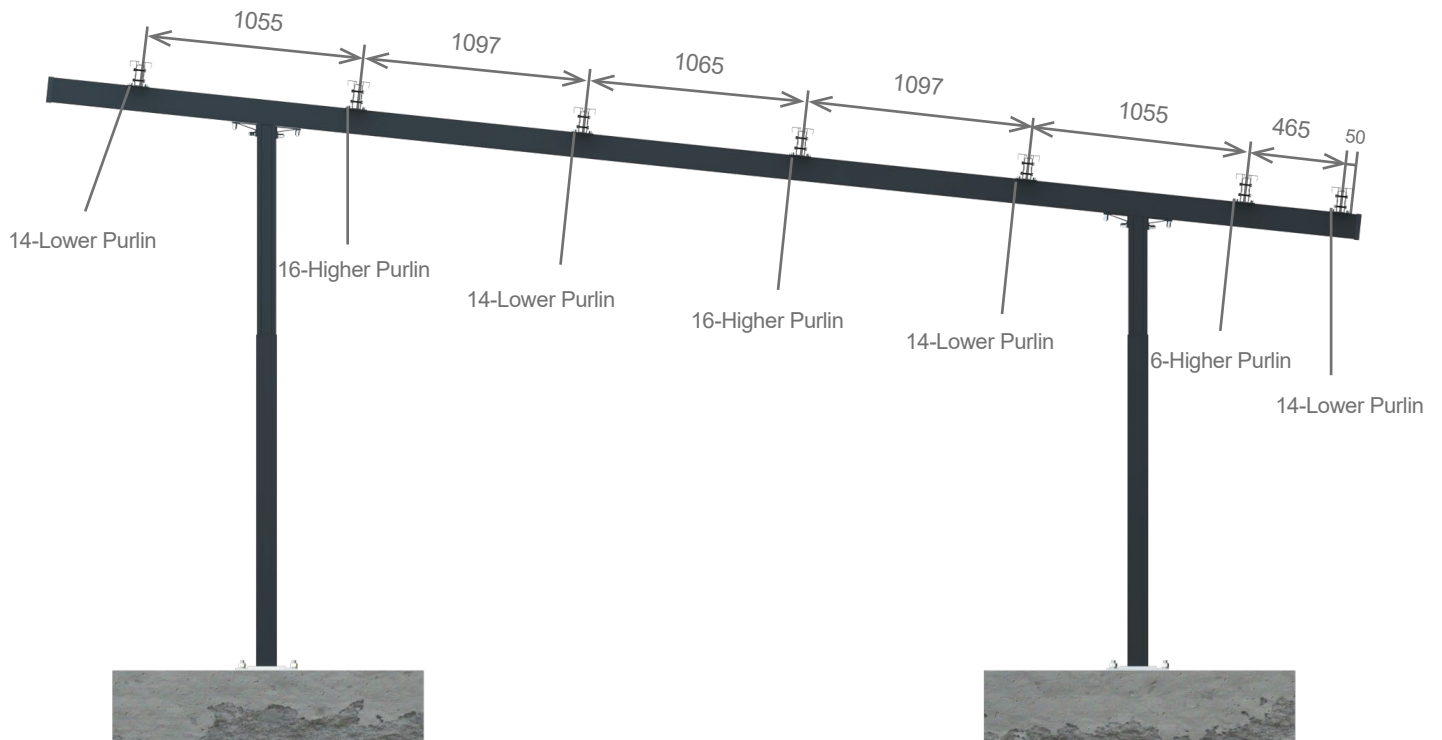
Purlin Spacing Diagram
