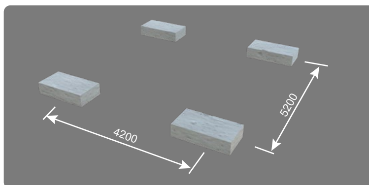
Foundation Layout Diagram
