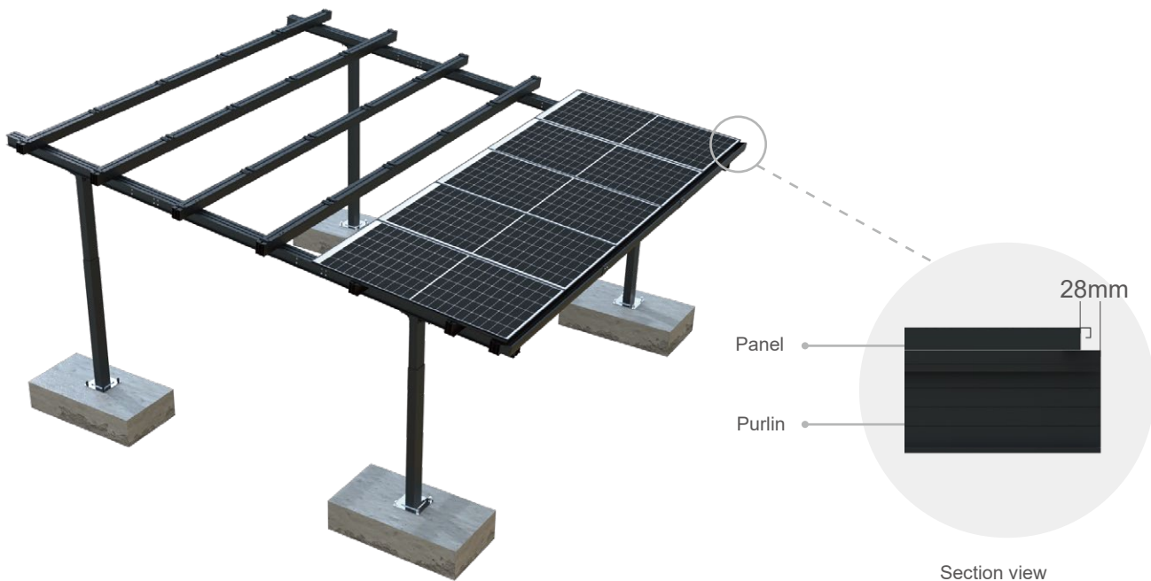
First Row Solar Panel Completion
